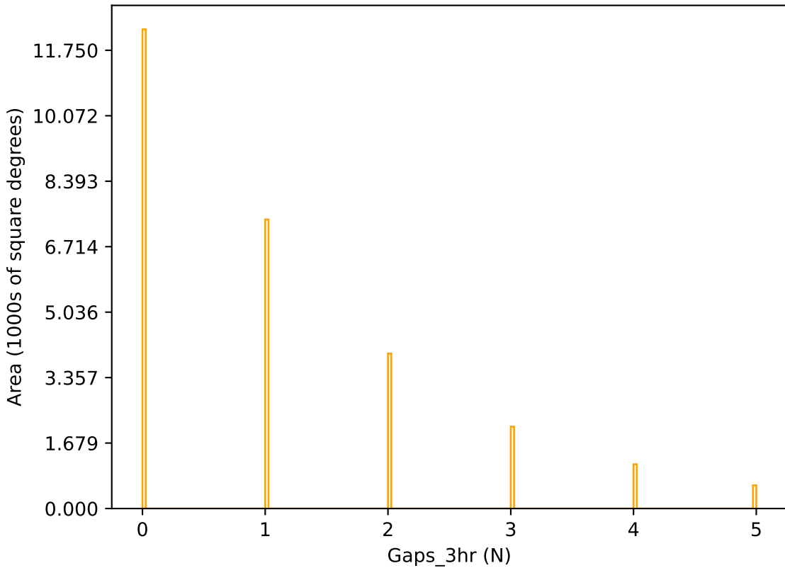
too_ignore_5_4v3.4_10yrs r band: Gaps_3hr
