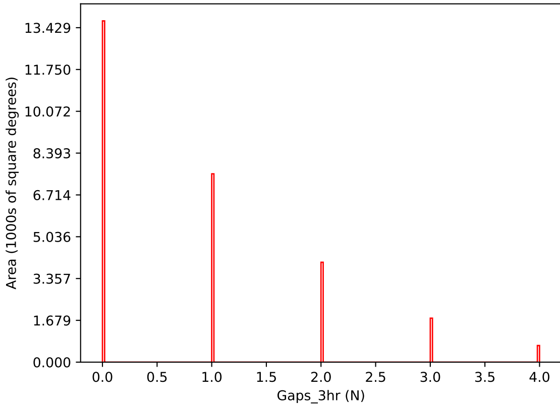
too_ignore_5_4v3.4_10yrs i band: Gaps_3hr
