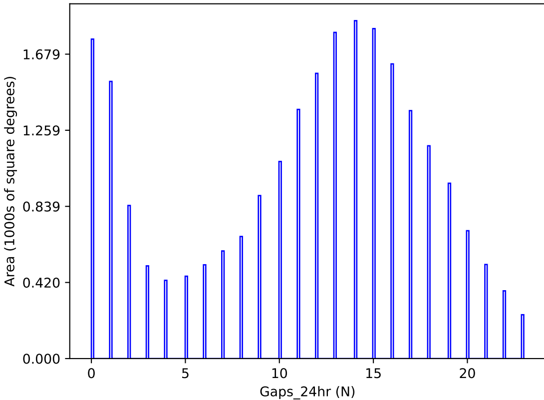
too_ignore_5_4v3.4_10yrs y band: Gaps_24hr
