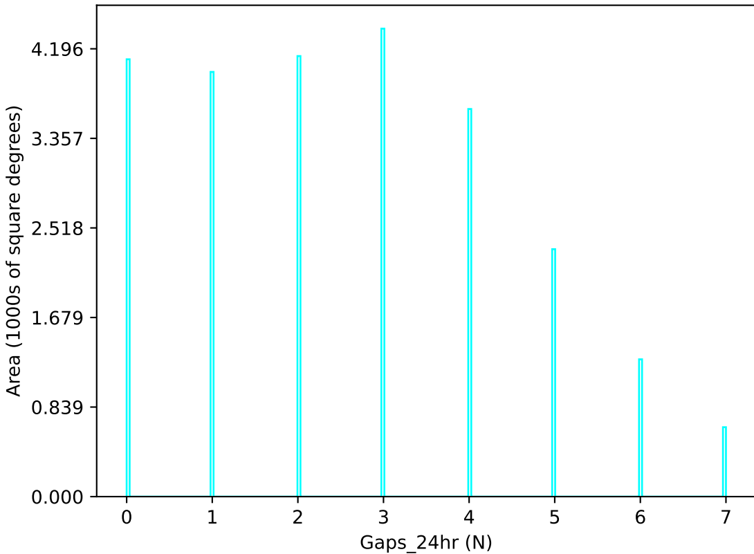
too_ignore_5_4v3.4_10yrs u band: Gaps_24hr
