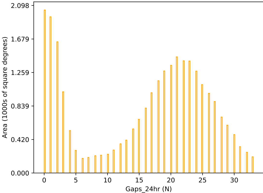
too_ignore_5_4v3.4_10yrs r band: Gaps_24hr
