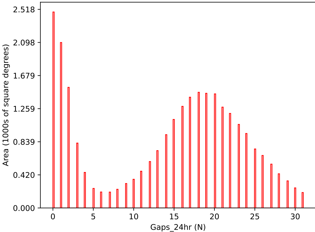
too_ignore_5_4v3.4_10yrs i band: Gaps_24hr
