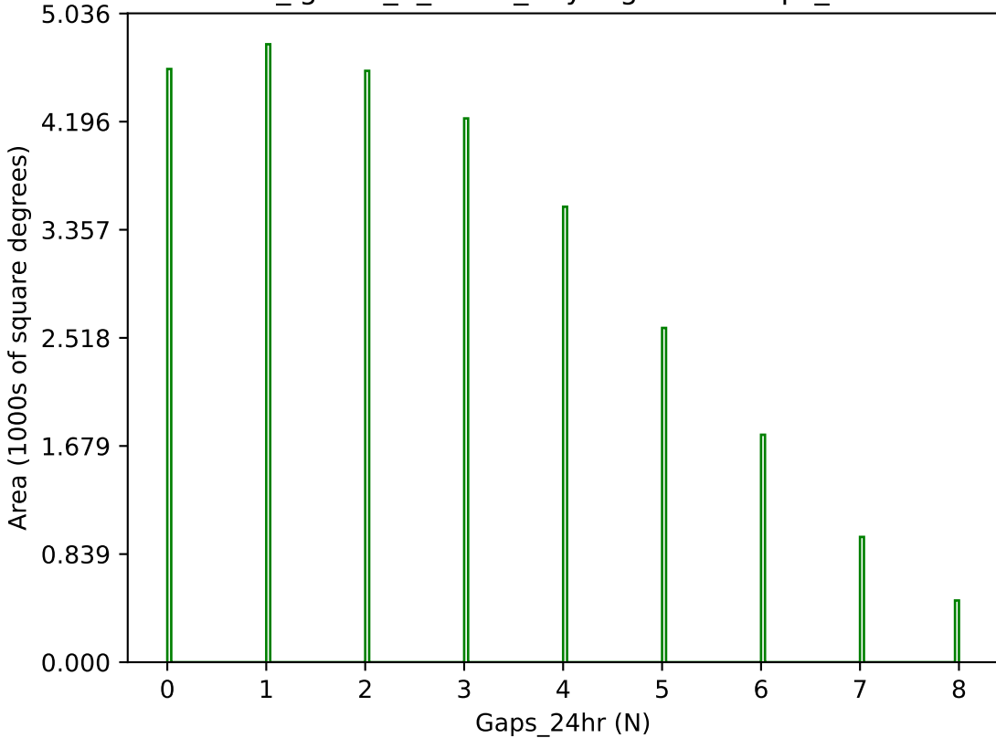
too_ignore_5_4v3.4_10yrs g band: Gaps_24hr
