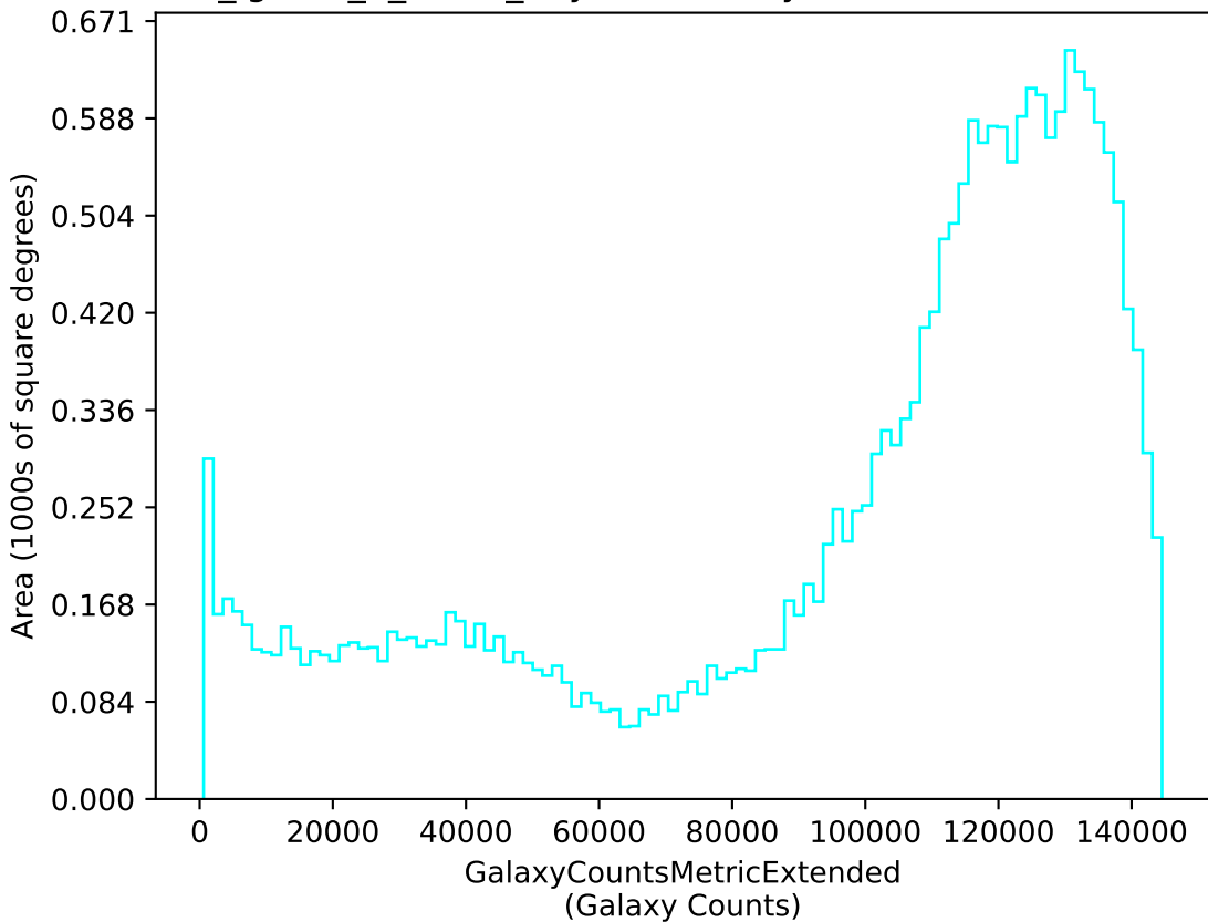
too_ignore_5_4v3.4_10yrs u: GalaxyCountsMetricExtended
