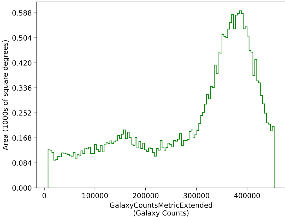
too_ignore_5_4v3.4_10yrs g: GalaxyCountsMetricExtended
