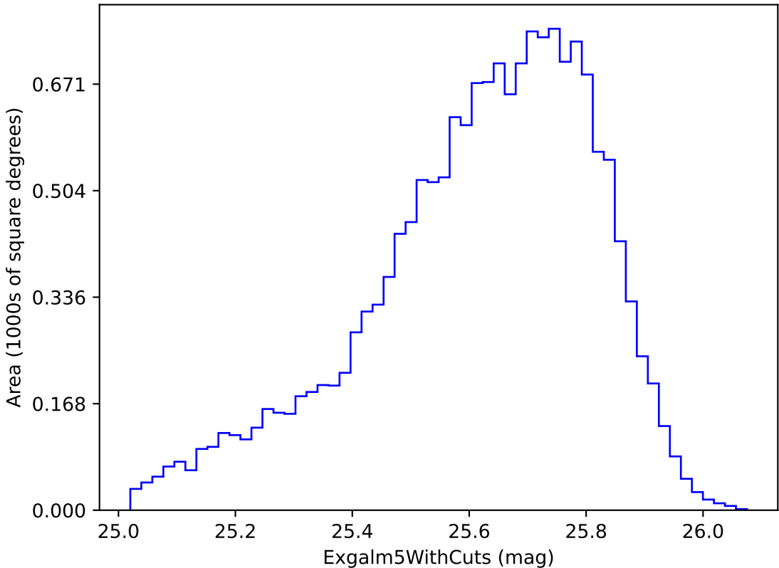
too_ignore_5_4v3.4_10yrs i band non-DD year 2: Exgal5WithCuts
