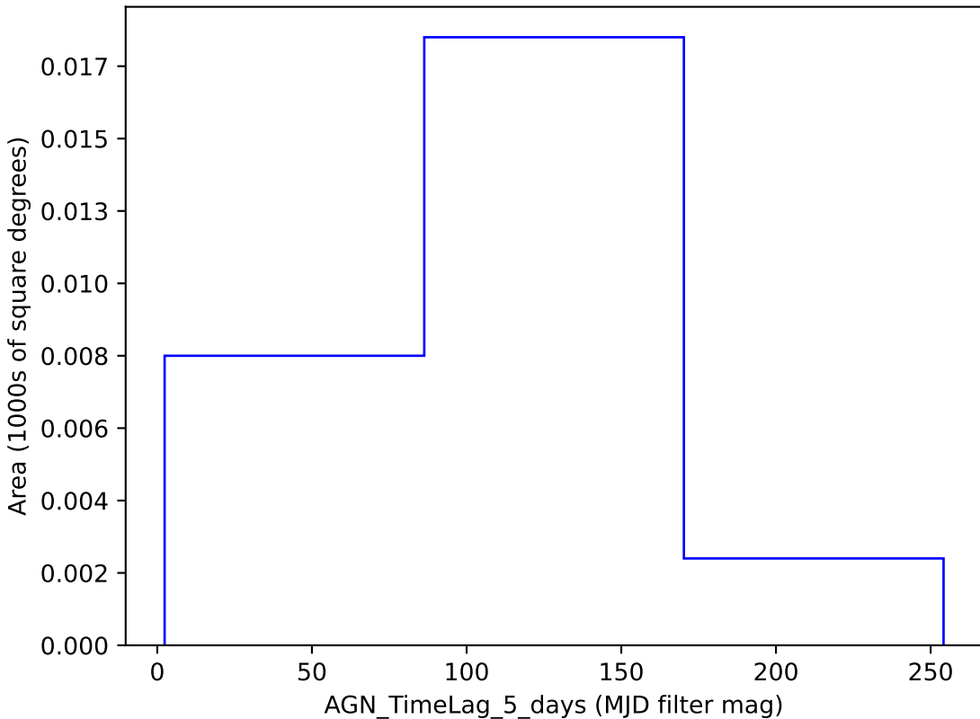
too_ignore_5_4v3.4_10yrs y band: AGN_TimeLag_5_days
