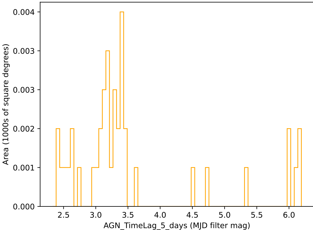
too_ignore_5_4v3.4_10yrs r band: AGN_TimeLag_5_days
