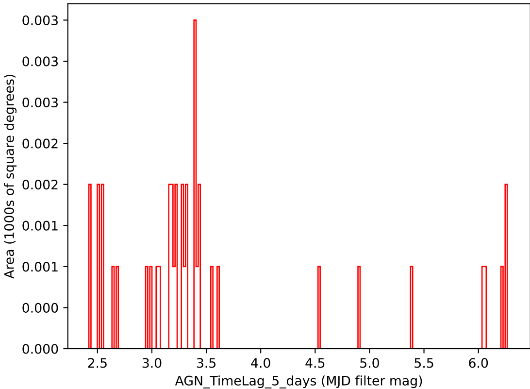
too_ignore_5_4v3.4_10yrs i band: AGN_TimeLag_5_days
