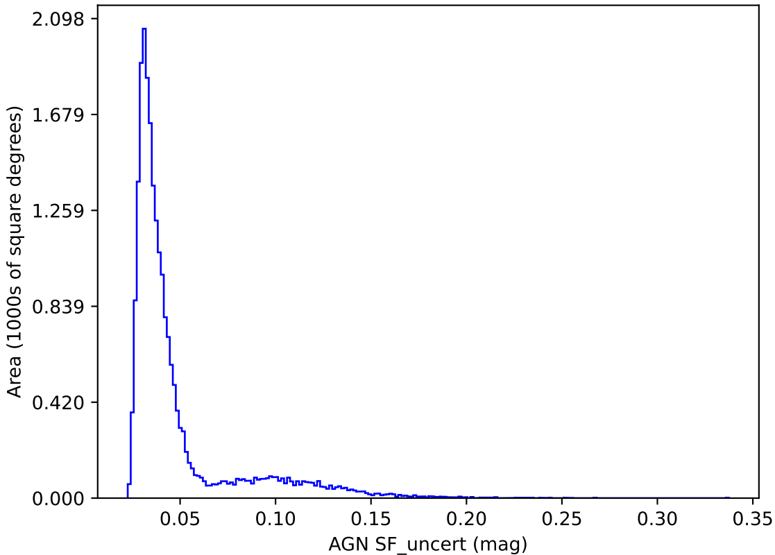
too_ignore_5_4v3.4_10yrs y band: AGN SF_uncert
