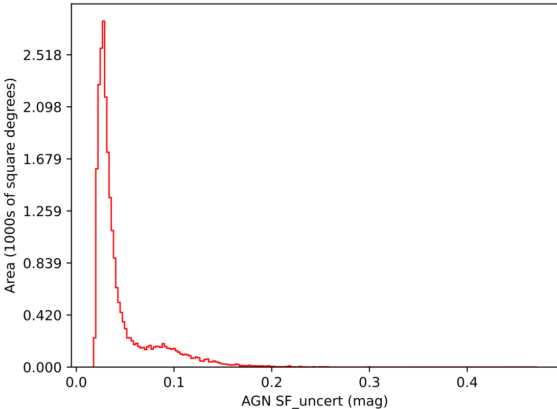
too_ignore_5_4v3.4_10yrs i band: AGN SF_uncert
