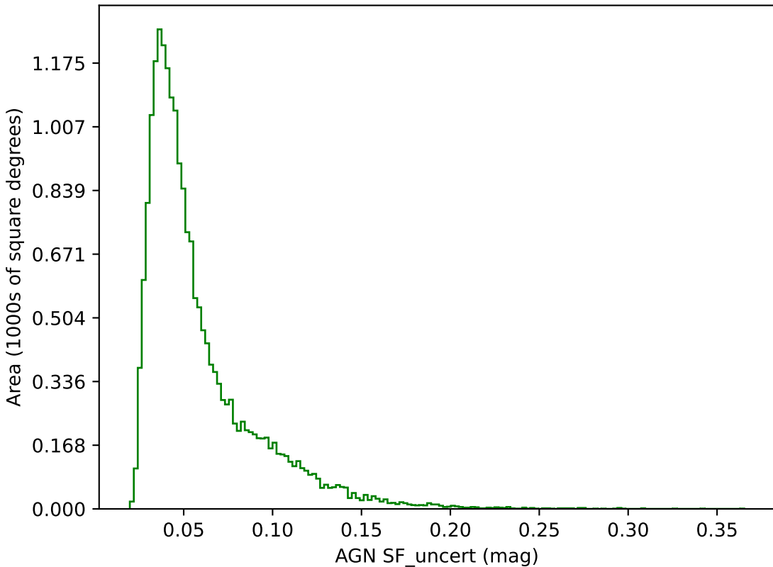
too_ignore_5_4v3.4_10yrs g band: AGN SF_uncert
