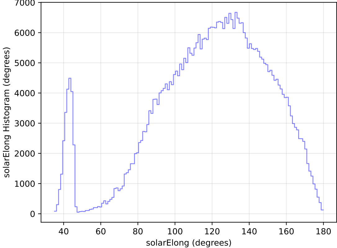
too_ignore_5_4v3.4_10yrs WFD z band: solarElong Histogram
