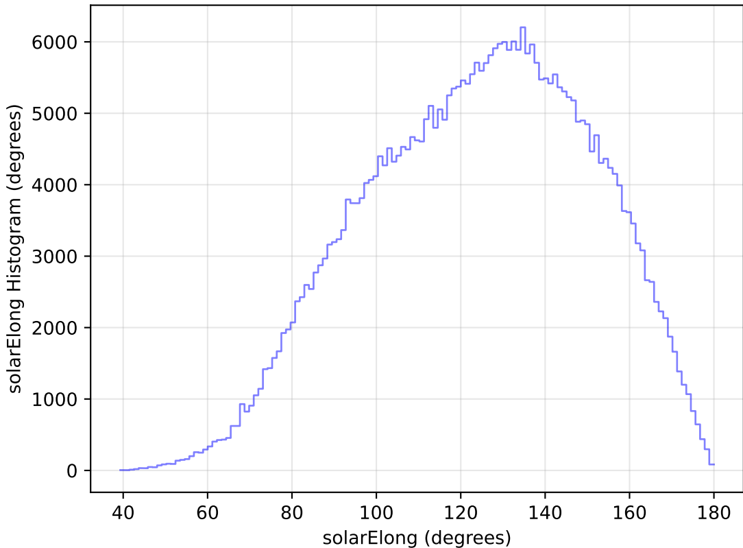
too_ignore_5_4v3.4_10yrs WFD y band: solarElong Histogram
