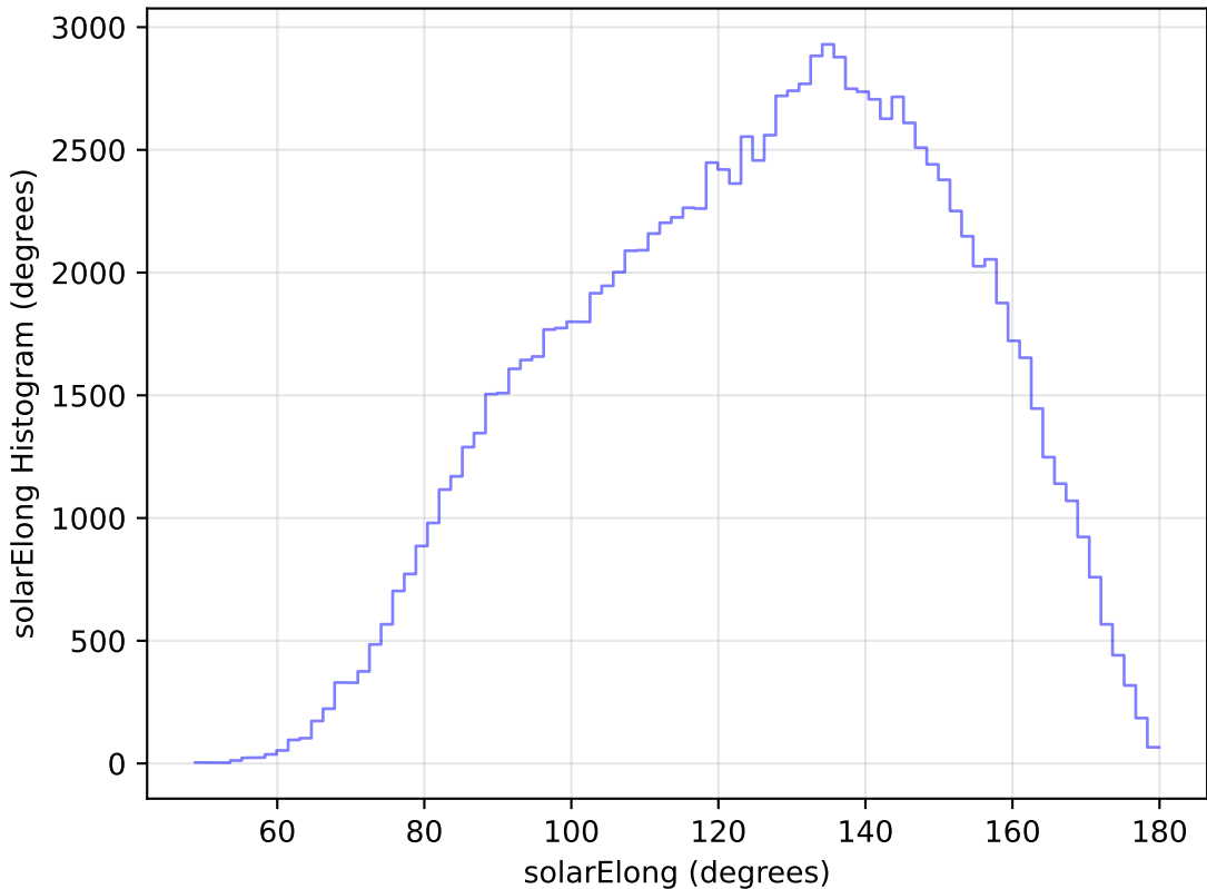
too_ignore_5_4v3.4_10yrs WFD u band: solarElong Histogram
