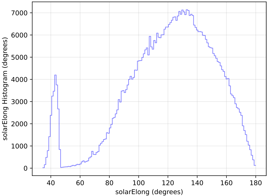
too_ignore_5_4v3.4_10yrs WFD i band: solarElong Histogram
