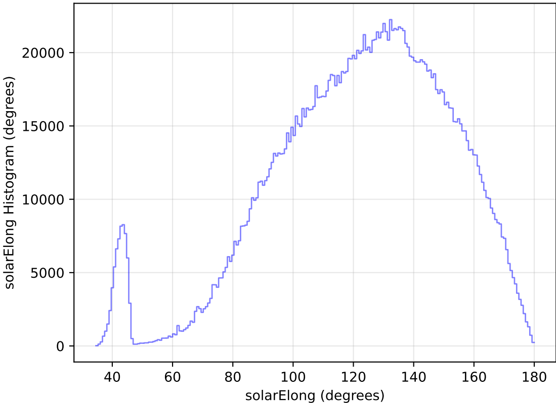
too_ignore_5_4v3.4_10yrs WFD all bands: solarElong Histogram
