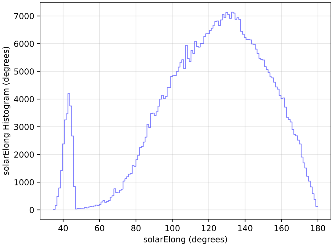
too_ignore_5_4v3.4_10yrs All sky i band: solarElong Histogram
