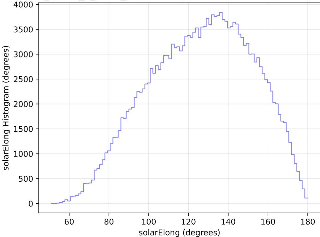
too_ignore_5_4v3.4_10yrs All sky g band: solarElong Histogram
