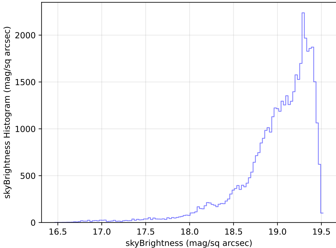
too_ignore_5_4v3.4_10yrs Yr 1 z band: skyBrightness Histogram
