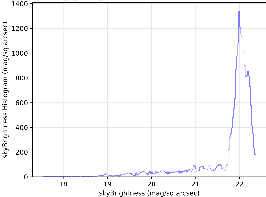
too_ignore_5_4v3.4_10yrs Yr 1 g band: skyBrightness Histogram
