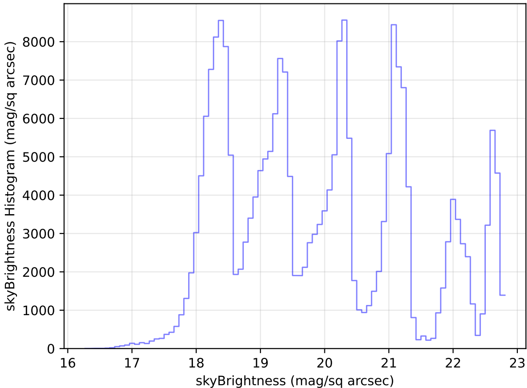
too_ignore_5_4v3.4_10yrs Yr 1 all bands: skyBrightness Histogram
