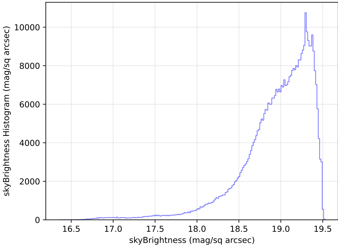
too_ignore_5_4v3.4_10yrs WFD z band: skyBrightness Histogram
