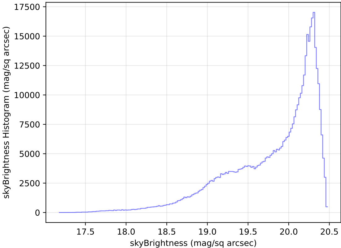
too_ignore_5_4v3.4_10yrs WFD i band: skyBrightness Histogram
