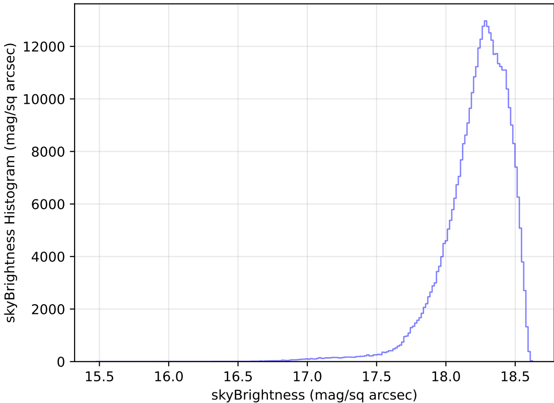
too_ignore_5_4v3.4_10yrs All sky y band: skyBrightness Histogram
