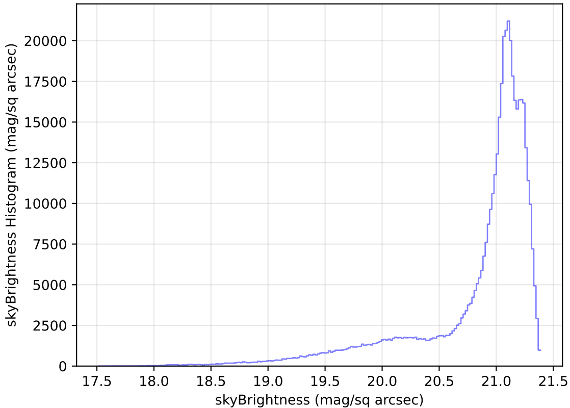
too_ignore_5_4v3.4_10yrs All sky r band: skyBrightness Histogram
