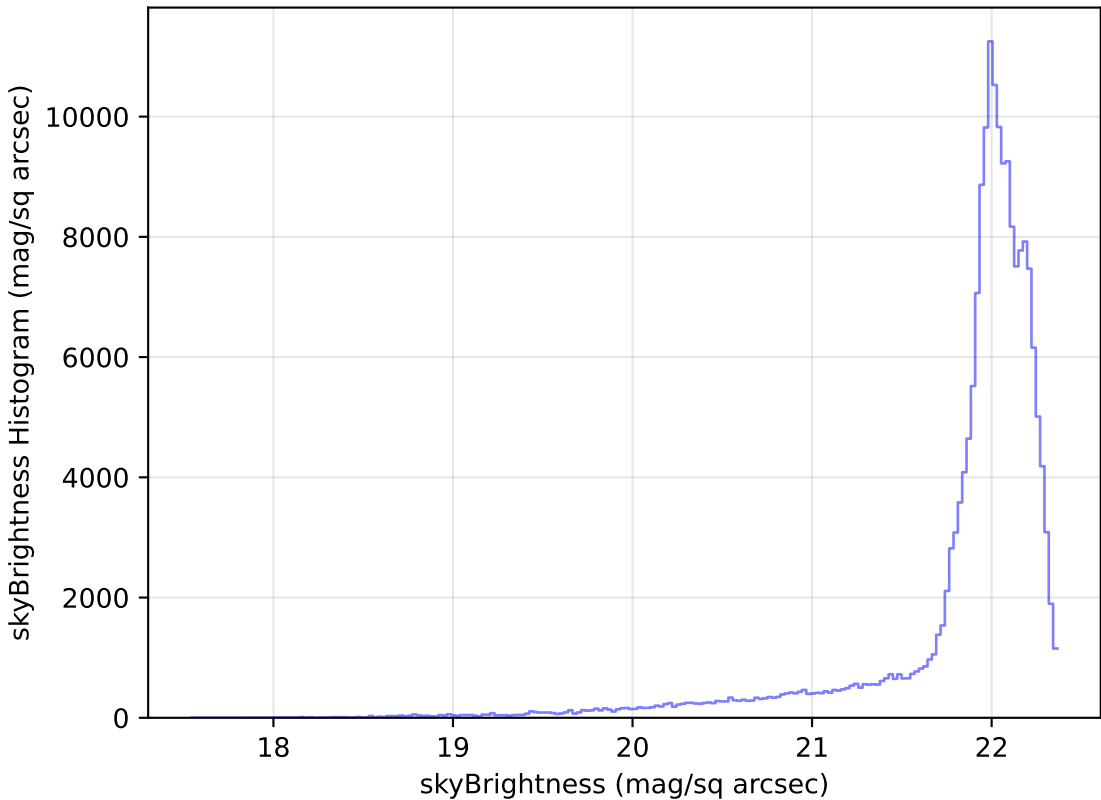
too_ignore_5_4v3.4_10yrs All sky g band: skyBrightness Histogram
