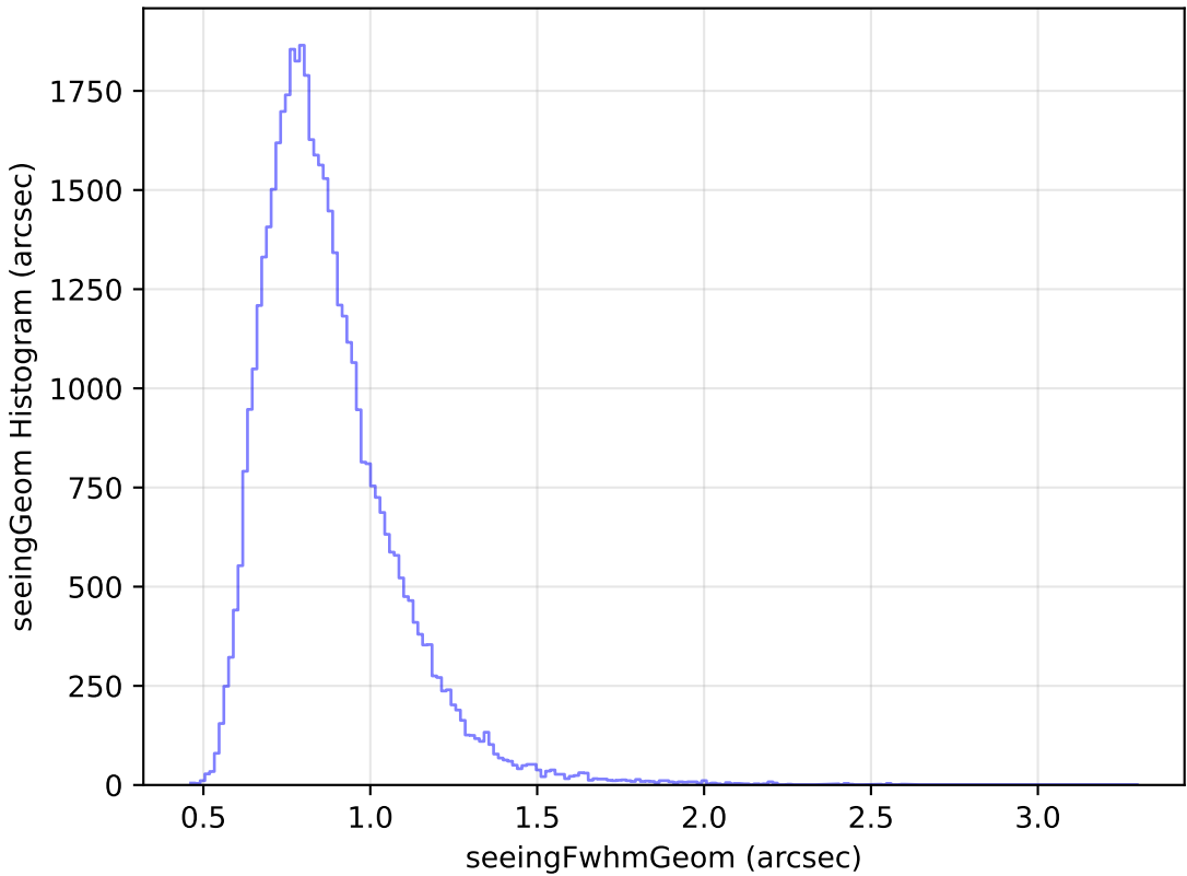
too_ignore_5_4v3.4_10yrs Yr 1 y band: seeingGeom Histogram
