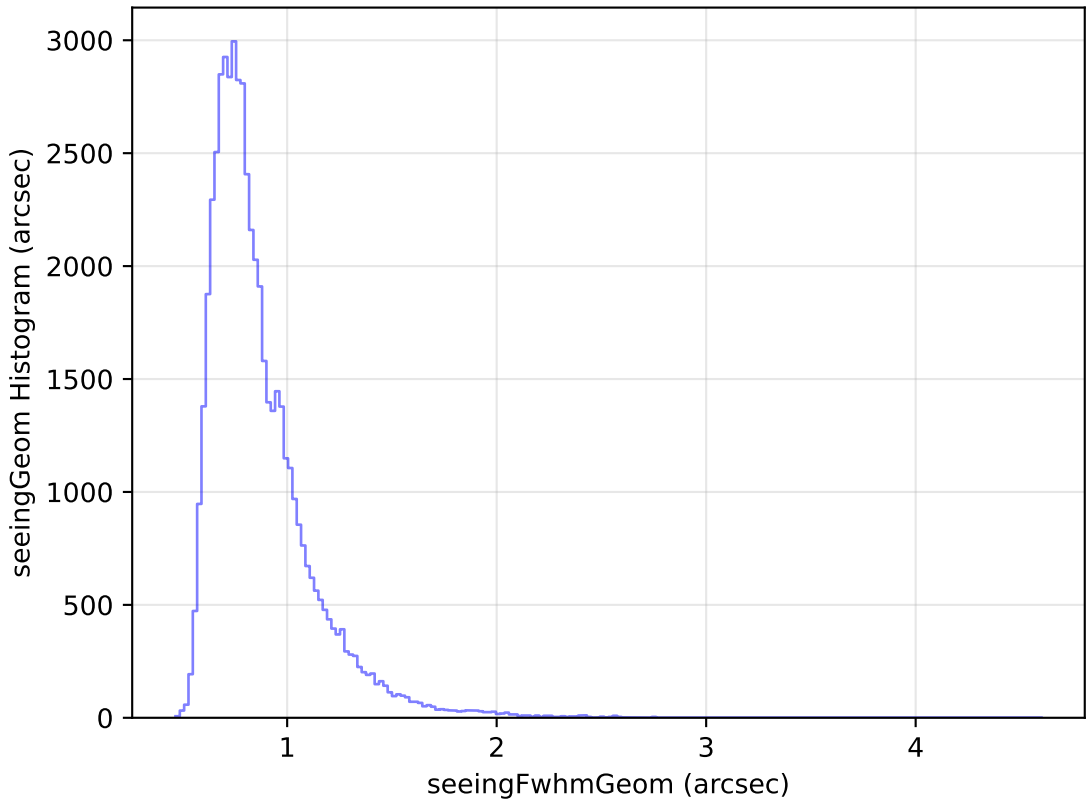
too_ignore_5_4v3.4_10yrs Yr 1 i band: seeingGeom Histogram
