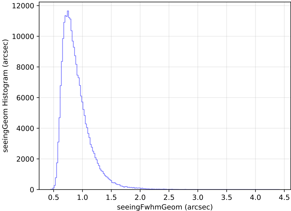
too_ignore_5_4v3.4_10yrs Yr 1 all bands: seeingGeom Histogram
