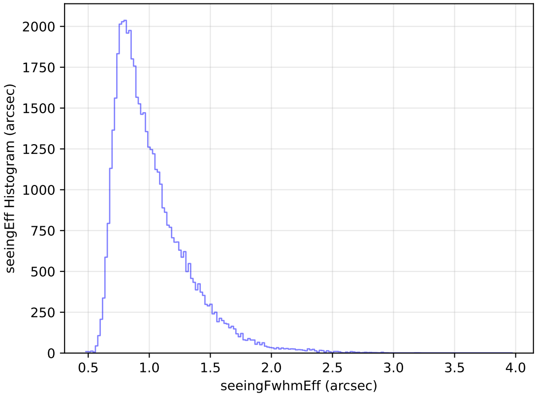
too_ignore_5_4v3.4_10yrs Yr 1 r band: seeingEff Histogram
