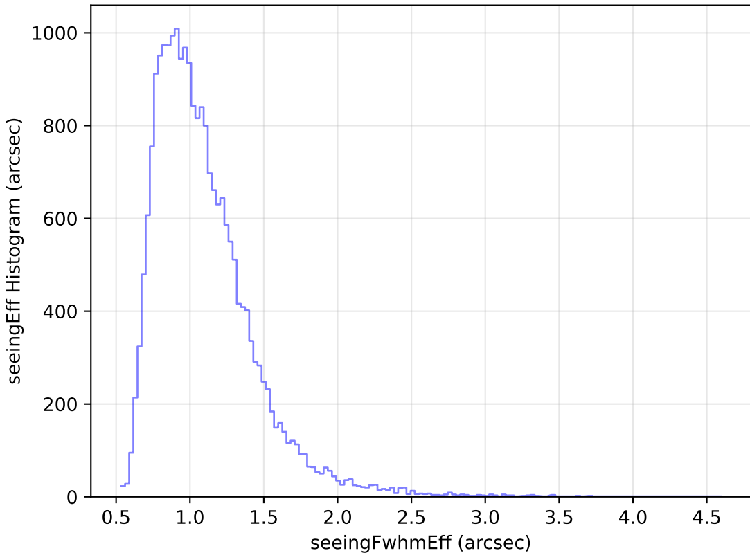
too_ignore_5_4v3.4_10yrs Yr 1 g band: seeingEff Histogram
