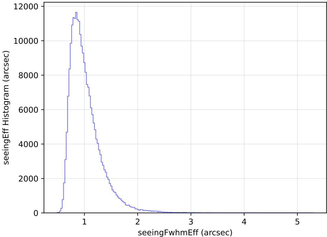
too_ignore_5_4v3.4_10yrs Yr 1 all bands: seeingEff Histogram
