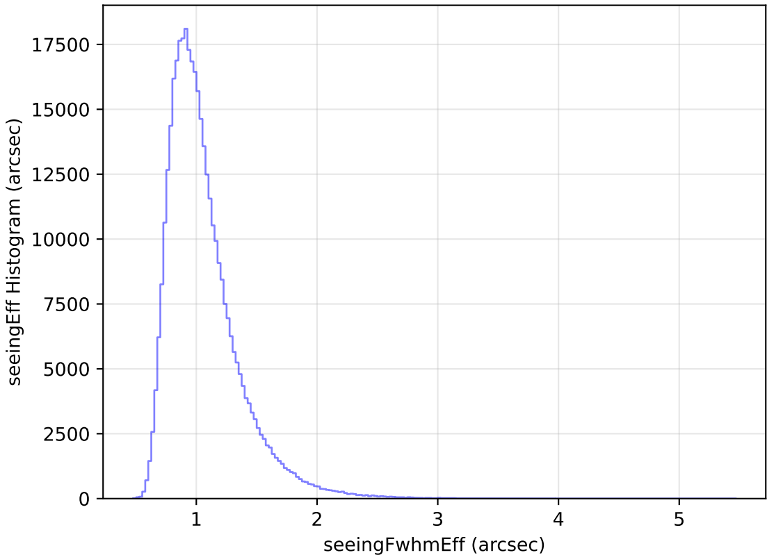
too_ignore_5_4v3.4_10yrs WFD y band: seeingEff Histogram
