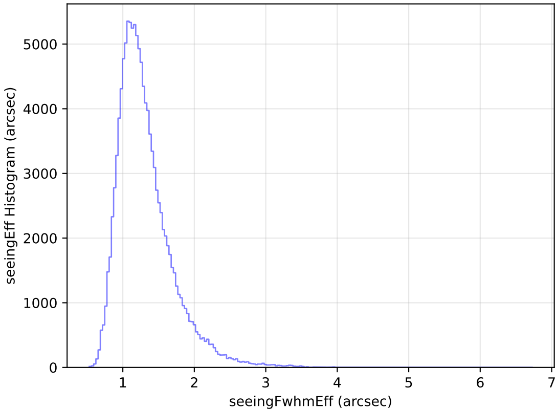
too_ignore_5_4v3.4_10yrs WFD u band: seeingEff Histogram
