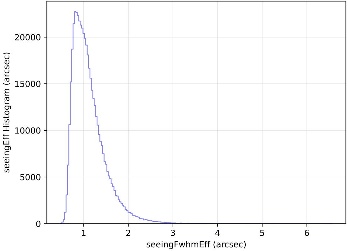
too_ignore_5_4v3.4_10yrs WFD r band: seeingEff Histogram
