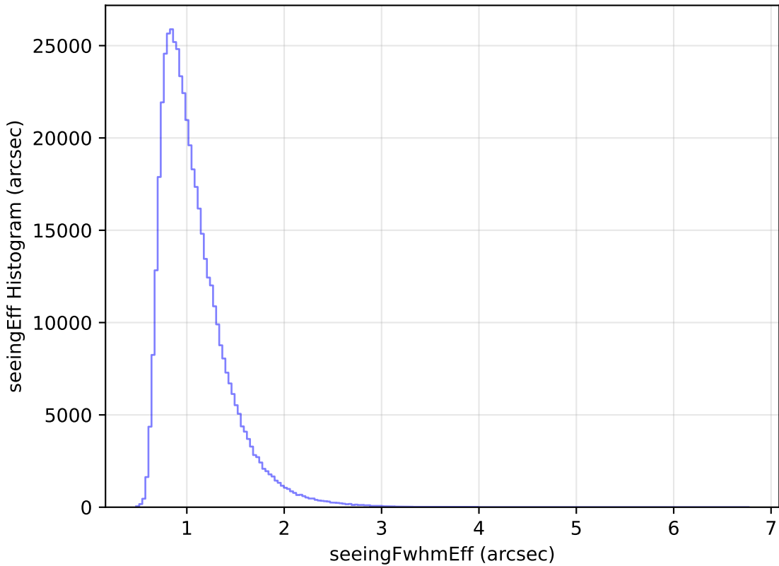
too_ignore_5_4v3.4_10yrs WFD i band: seeingEff Histogram
