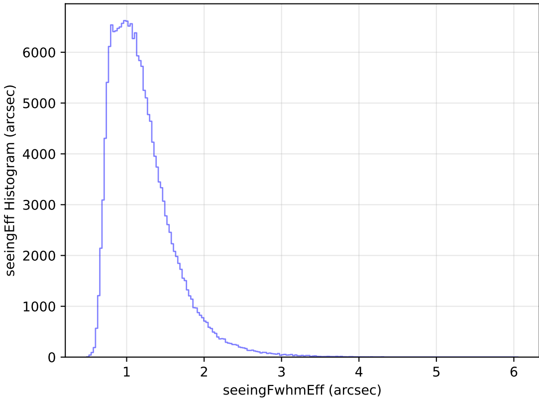
too_ignore_5_4v3.4_10yrs WFD g band: seeingEff Histogram
