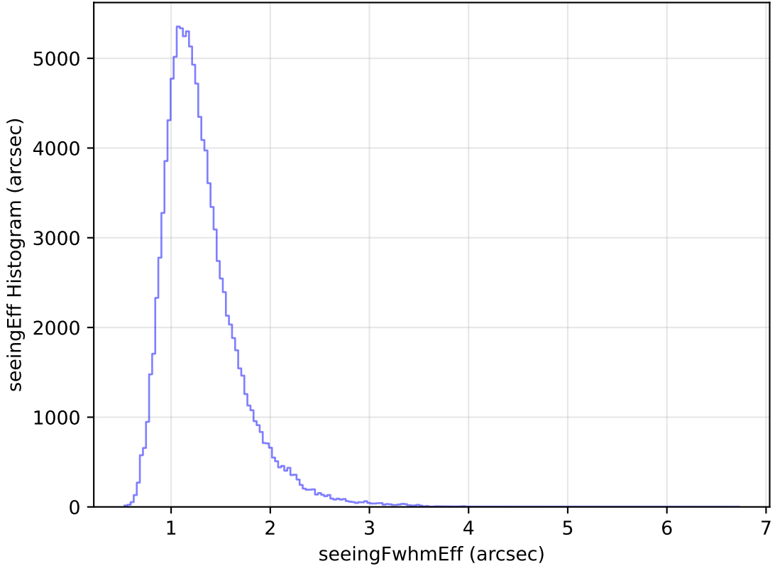
too_ignore_5_4v3.4_10yrs All sky u band: seeingEff Histogram
