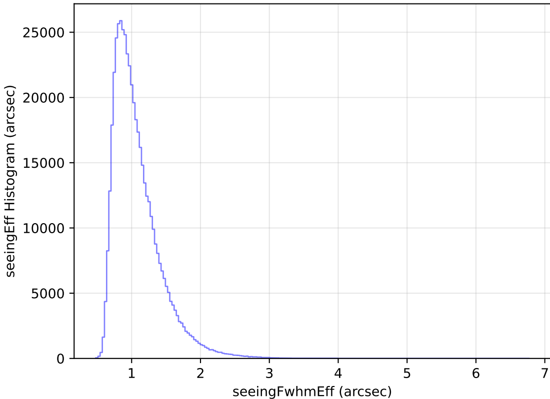
too_ignore_5_4v3.4_10yrs All sky i band: seeingEff Histogram
