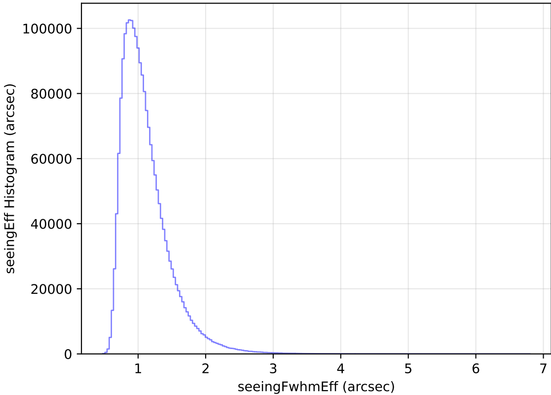
too_ignore_5_4v3.4_10yrs All sky all bands: seeingEff Histogram
