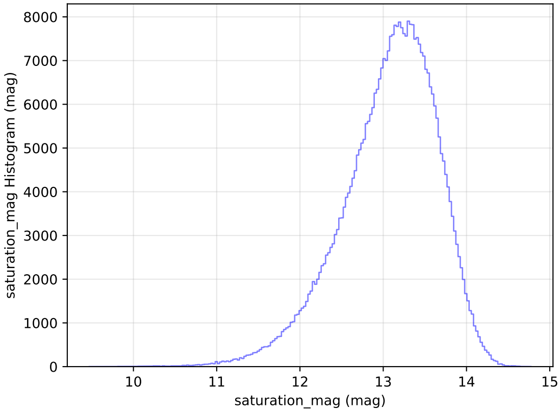
too_ignore_5_4v3.4_10yrs WFD y band: saturation_mag Histogram
