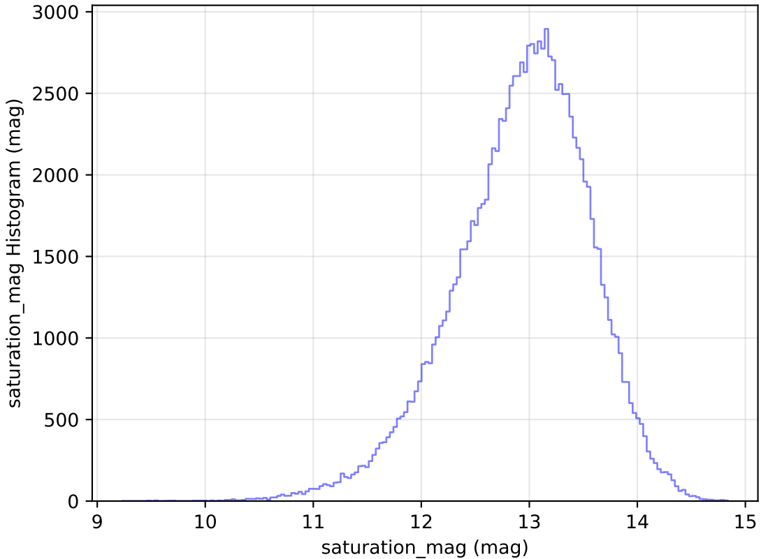
too_ignore_5_4v3.4_10yrs WFD u band: saturation_mag Histogram
