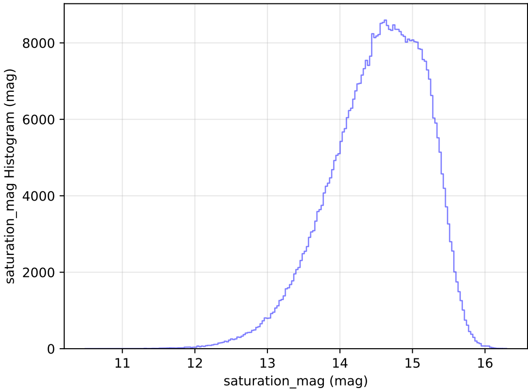
too_ignore_5_4v3.4_10yrs WFD r band: saturation_mag Histogram
