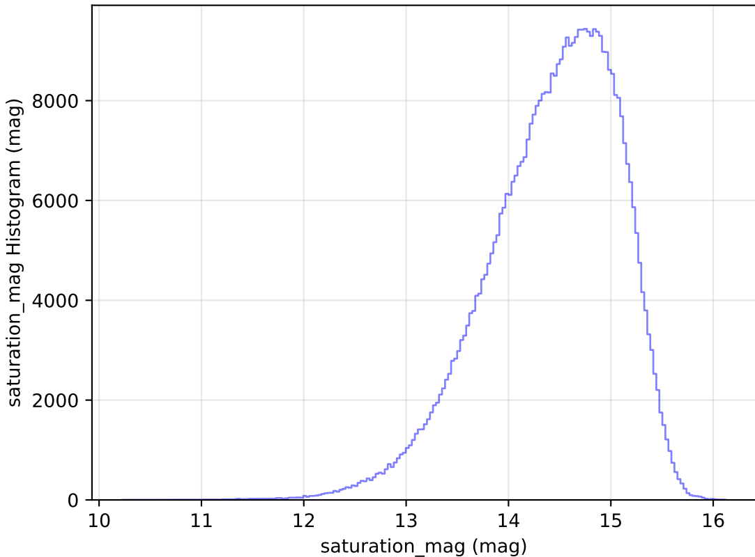
too_ignore_5_4v3.4_10yrs WFD i band: saturation_mag Histogram
