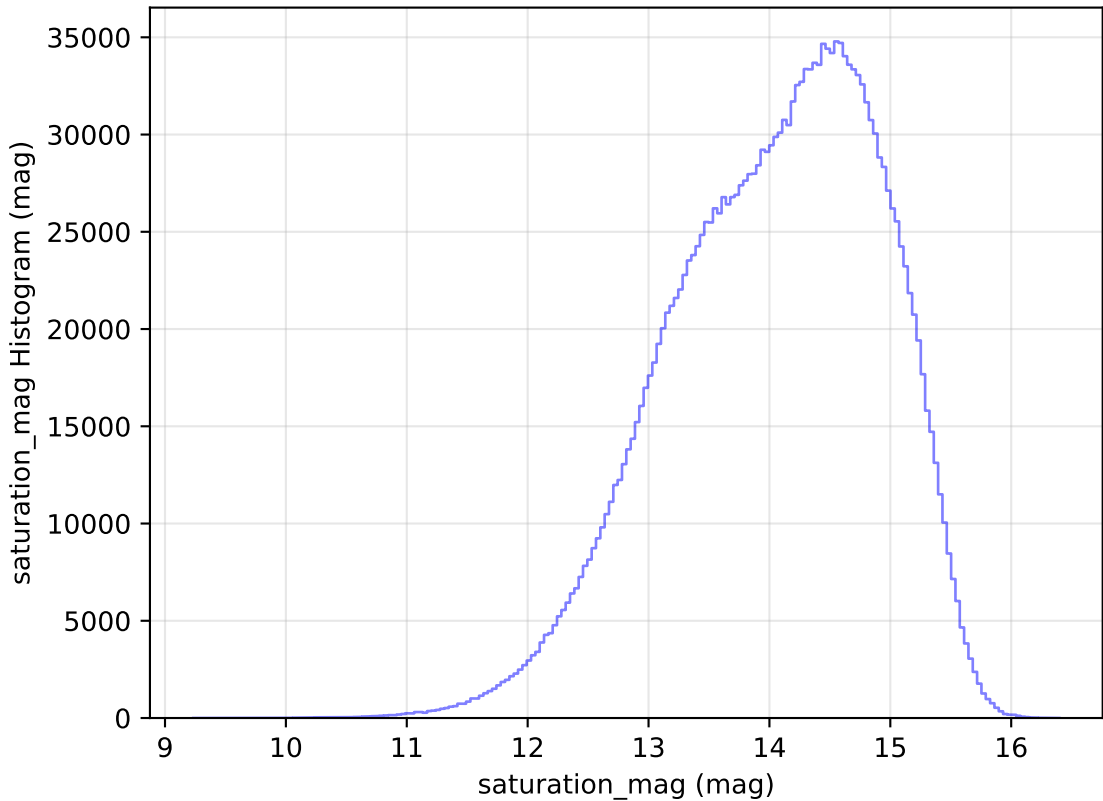
too_ignore_5_4v3.4_10yrs WFD all bands: saturation_mag Histogram
